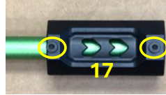
MS-03-229-A Gun Silencer Head Screw ( #17) - \phi 4 \times 28 \times M3
